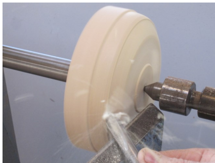
1. Turn the outside shape between Centres from both sides.
